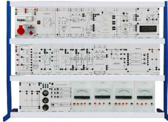
POWER ELECTRONICS TRAINING KIT Model GOTT-PET-588A
