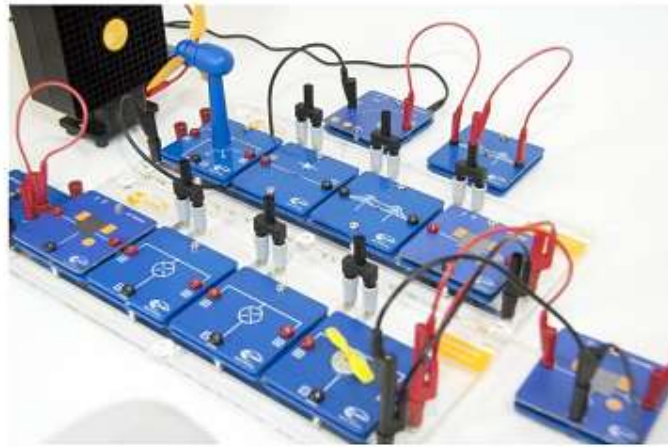
leXsolar-SmartGrid Professional
